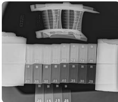
Aircraft blade casting
