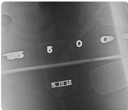
Carbon steel pipe weld
